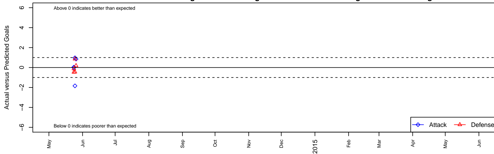
AC Samoa Tens G03 Dots are actual minus expected GF (blue circles) and GA (red triangles). Blue line is smoothed change in attack strength. Red is smoothed change in defense strength.
